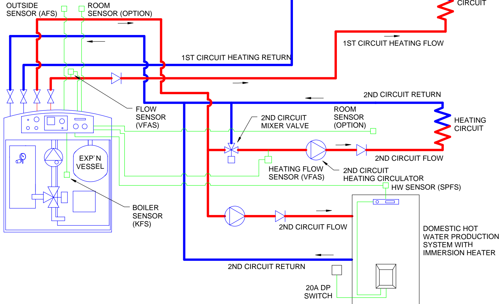
FCX BOILER CONNECTION TO A DOUBLE HEATING CIRCUIT, DOMESTIC HOT WATER PRODUCTION SYSTEM WITH IMMERSION HEATER
